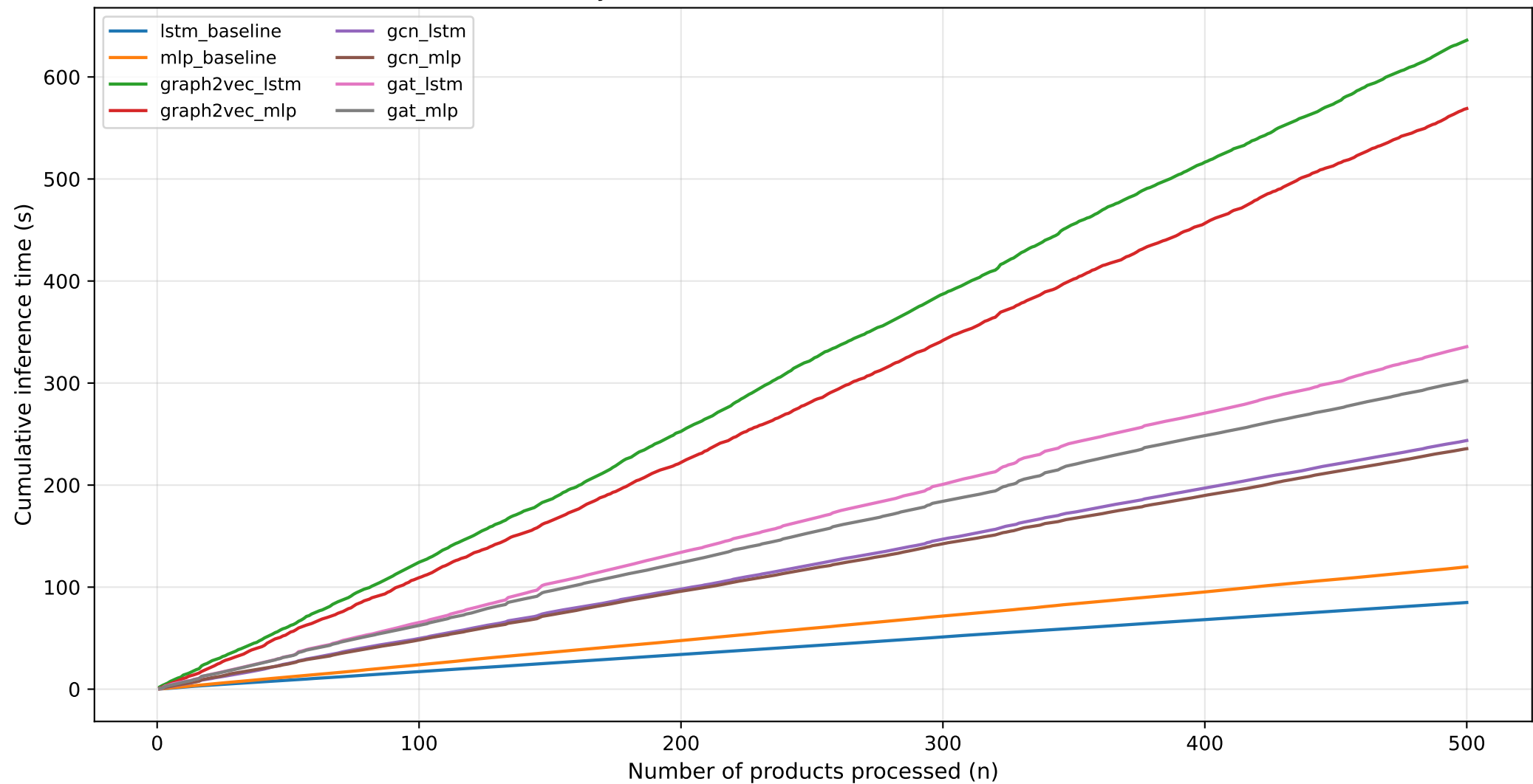
Scalability: cumulative inference time vs workload size
